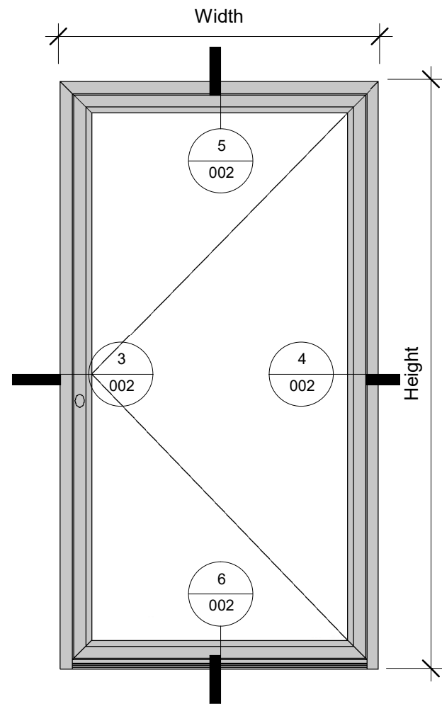
1 Elevation Front 1 : 20
